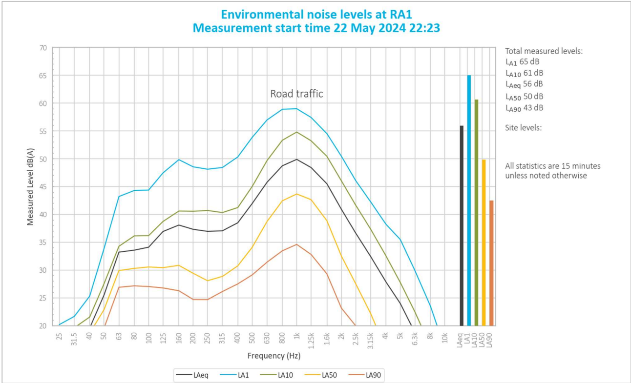
Figure 5.6 Environmental noise levels – RA1 (Pacific Highway) – Night
