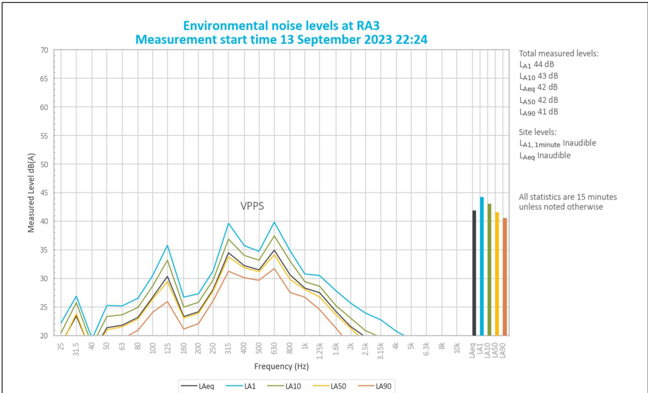
Figure 5.5 Environmental noise levels – RA3, Kingfisher Shores
